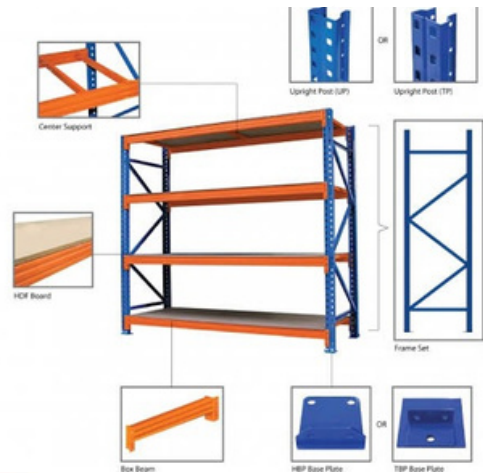
PE-87 HEAVY DUTY STORAGE RACK
